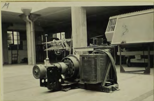
DYNAMOMETER MOTOR Motor laboratory UNI. OF MUNICH
