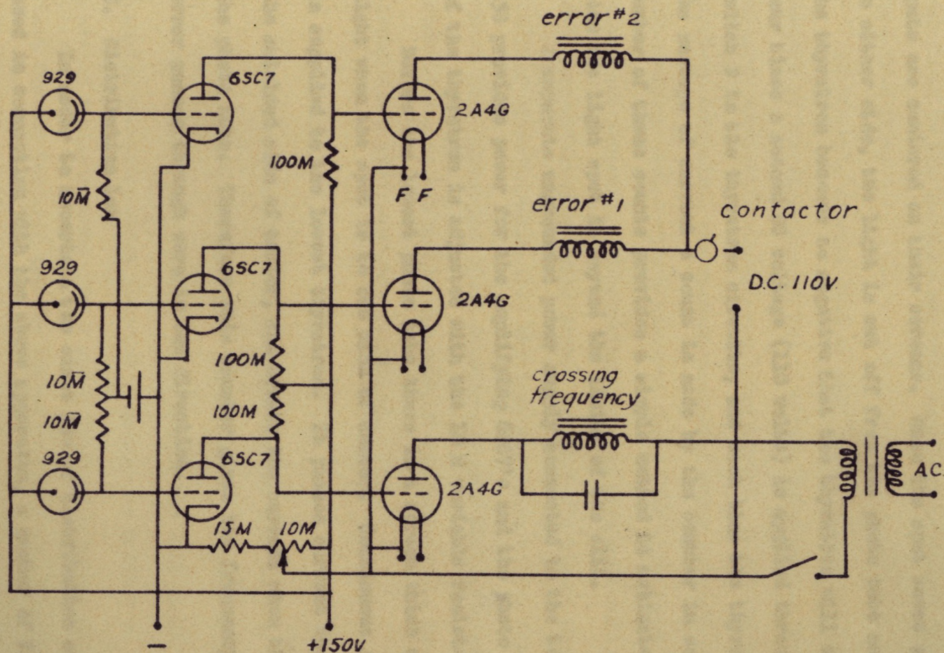
Counter Circuit
