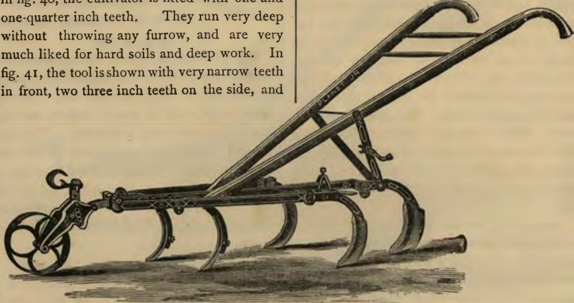
Fig. 41.—The "Planet Jr." Cultivator, showing different angles at which the Teeth can be set.
