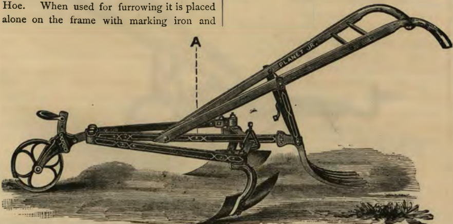
Fig. 35.—The "Planet Jr." Horse Hoe with Rake Covering Attachment. Rake, Price, $1.25.
