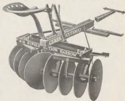
This 8-Disk Harrow is Popular in the South for Use with Two Light Mules. Note the Solid Disks
