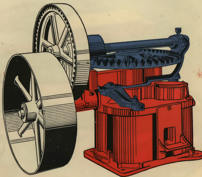
CHATTANOOGA CANE MILL—WITH BELT POWER ATTACHMENT
