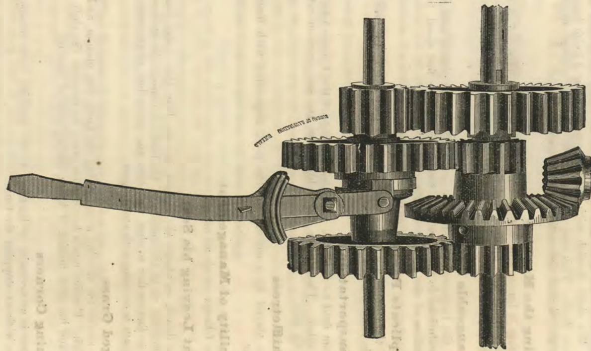
CHANGEABLE SPEED GEARING.
