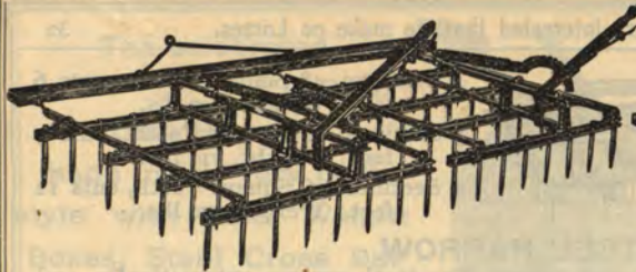
FLEXIBLE FRAME SHOWING SPRING.
