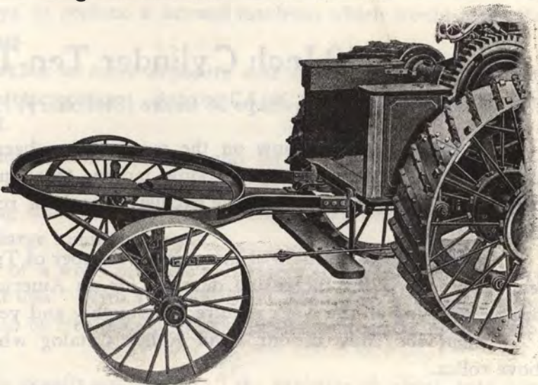
Tank Removed to Show Trucks, Frame and Coupling to Engine Platform.
