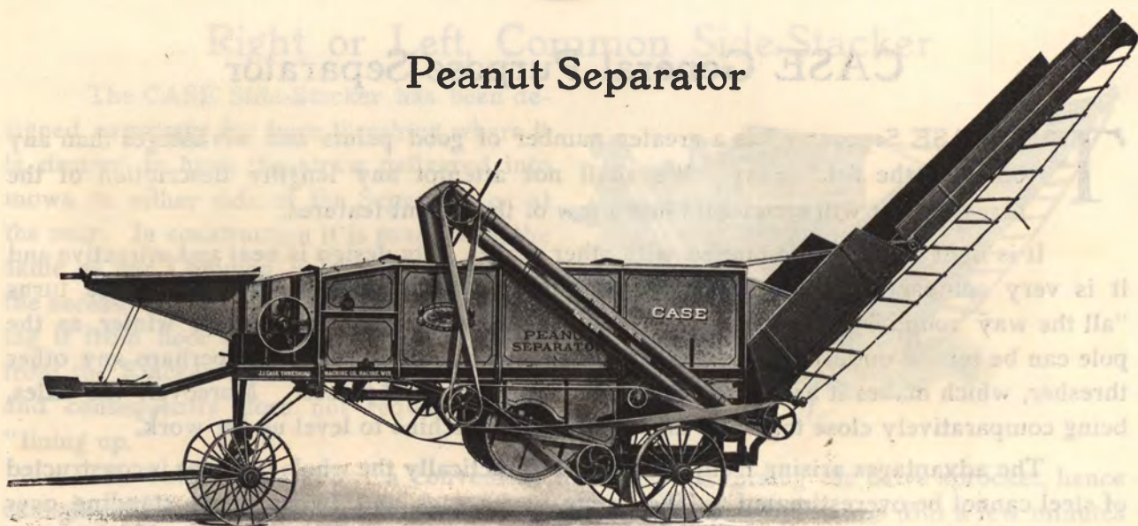
Right Side of the CASE Peanut Separator
