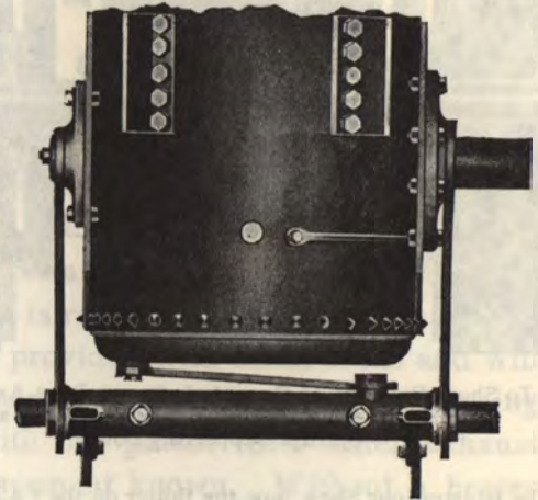
Showing Cross-Link and Stud Bearing to Prevent Side Play of Boiler.
