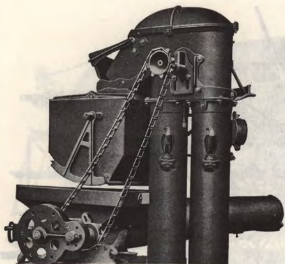
Head of Regular Weigher Showing Hopper, Conveyor and Chain Drive for Auger
