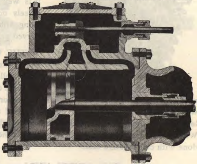
Sectional View of Simple Cylinder
