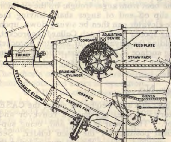
Interior View of Straw Bruiser and Shredder
