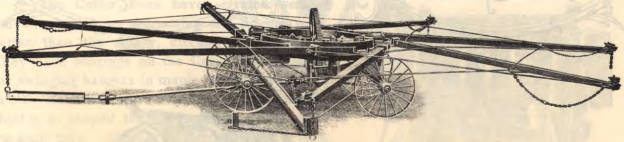
14 Horse-Power with Sweeps, Equalizer and Brace Rods and Tumbling Rods in Position, Platform Removed. Also built for 6, 8, 10 and 12 Horse-Power.
