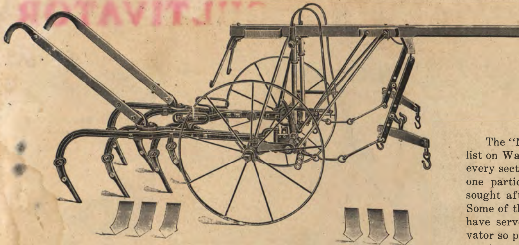
Showing Equipment of Six-Shovel Regular Gang. Pin Trip Cultivator- Single Tongue
