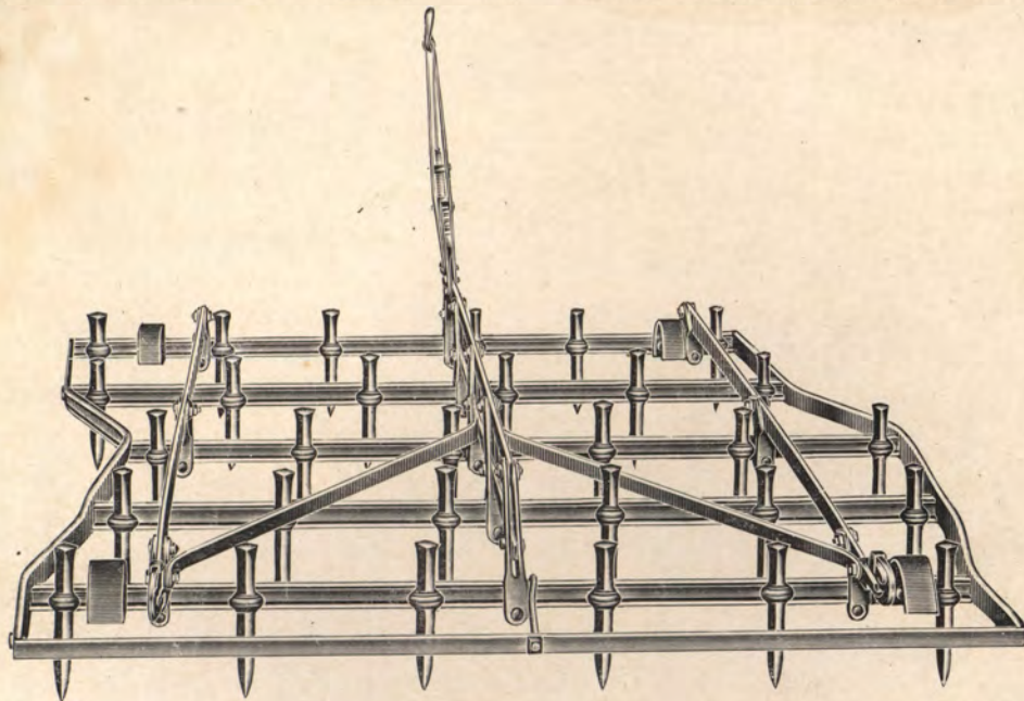
No. 2 Columbian "U Bar" Steel Lever Harrow.
