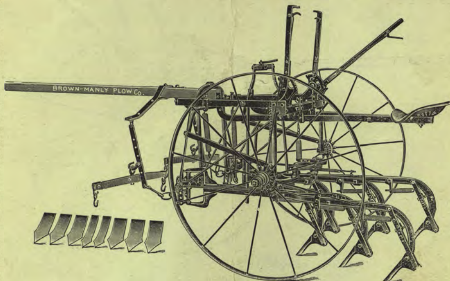
Showing Six-Tooth Regular Spring-Trip Gangs Made with either Round Boot or Slot Boot.
