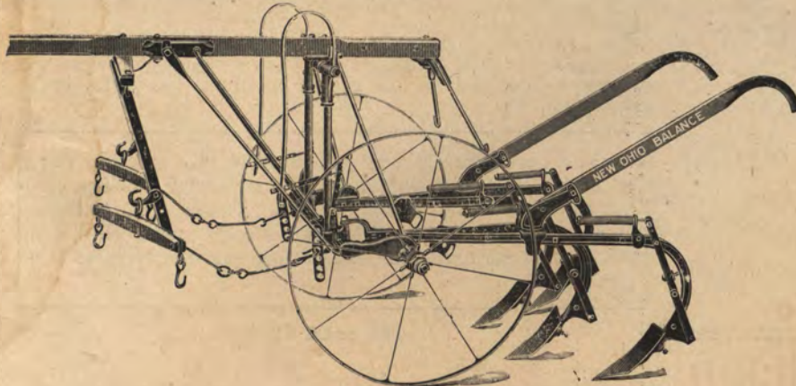
New Balance with Regular Spring-Trip Gangs
