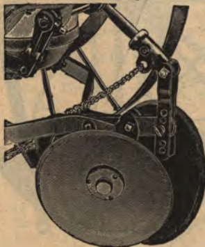
Fig. 218 Showing Double Disc Opening Plow.
