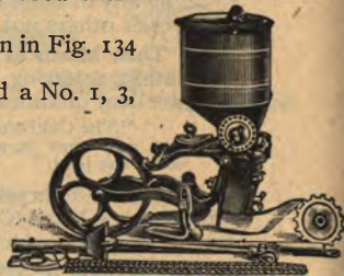
Fig. 134 No. 6 "Iron Age" Hill and Drill Seeder Attachment. Price, $5.00
