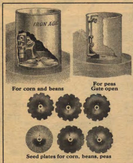
Fig. 267 Corn, bean and pea attachment. Price, complete, $6.25
