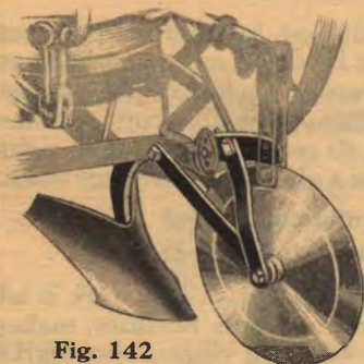
Fig. 142 Single disc opening plow, shown by solid parts. Price, attachment only, $4.75
