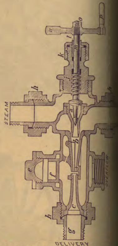
Sectional View of Peerless Injector
