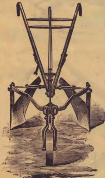
The Planet, J., Furrower, Ridger, &c — Making up Beds.
