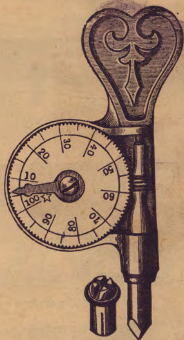
Speed Indicator.
