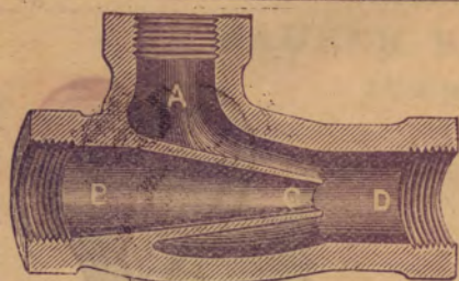
Suction Tee.
