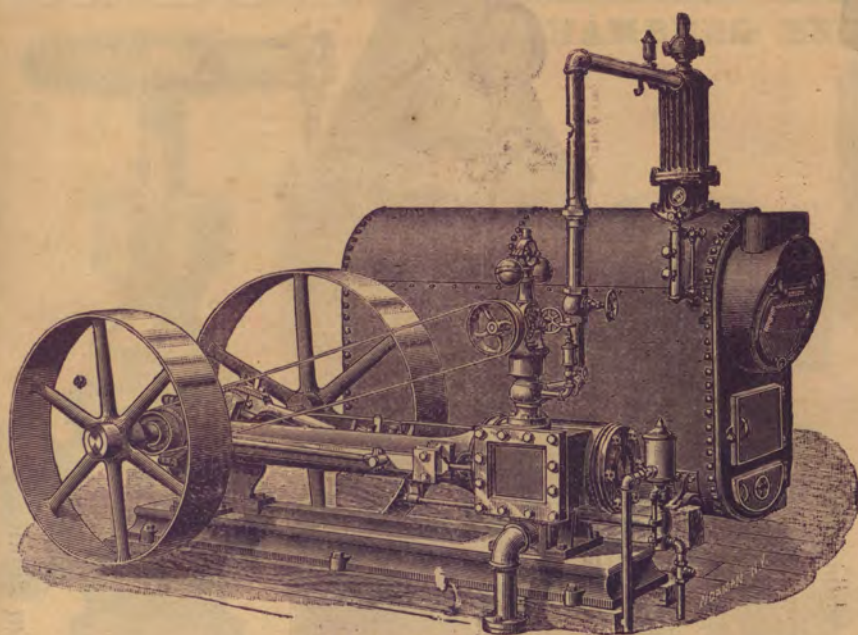
Horizontal Engine.
