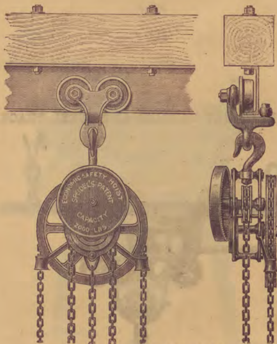
OVERHEAD TRAMWAY, With Trolley Running on Channel Beams.
