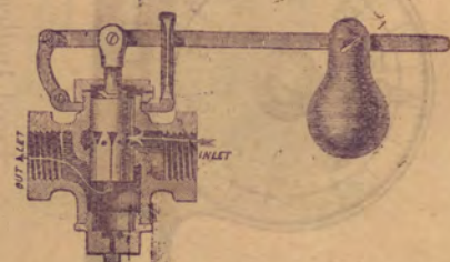
Steam Pump.
