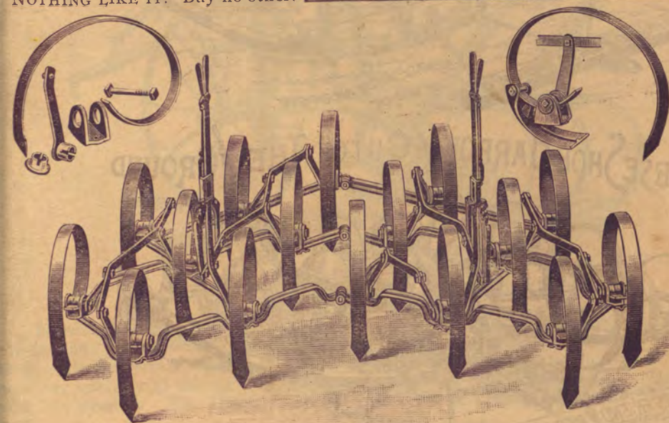
THE STEVENS LEVER HARROW, With Independent Tooth Adjustment. Has Elevated Cross Bars.
