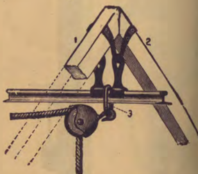
This shows pulley fastened in rear of mow when rope is taken down at gable end of barn.
