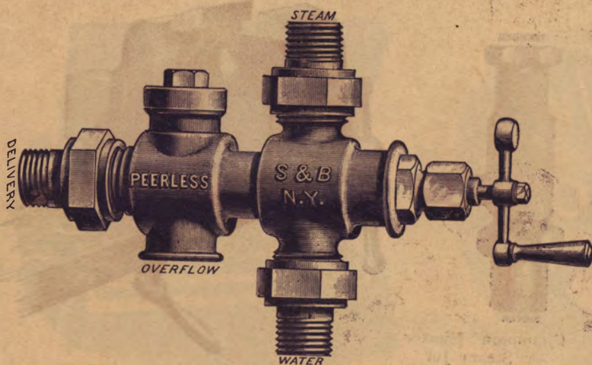
The Peerless Injector.
