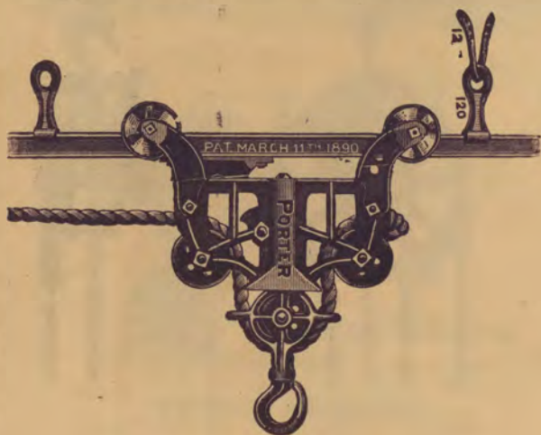
This shows pulley fastened in rear of mow when rope is taken down at gable end of barn.
