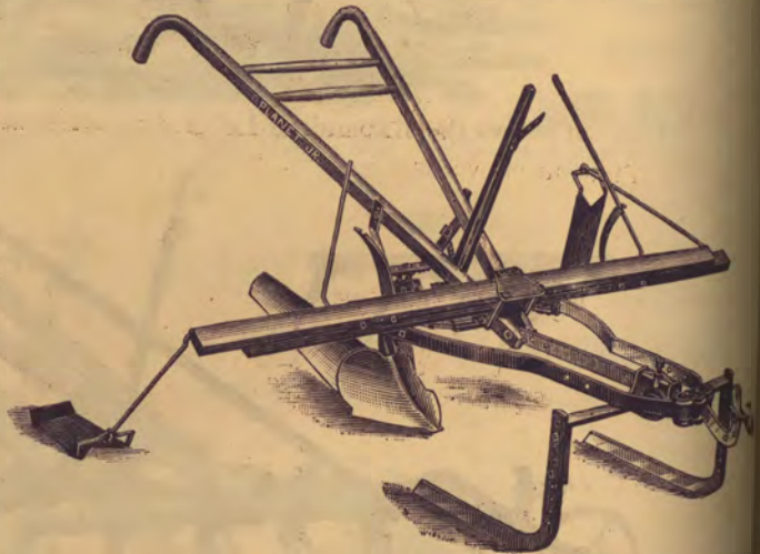
The Planet, Jr., combined Furrower, Marker, Hiller and Ridger.
