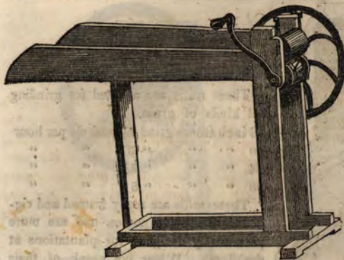
FIG. 41. CYLINDRICAL STRAW-CUTTER.
