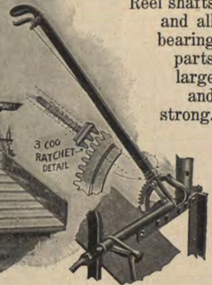
THE THREE-COG RATCHET LEVER
