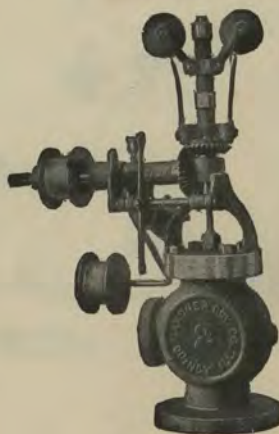
GARDNER GOVERNOR.
