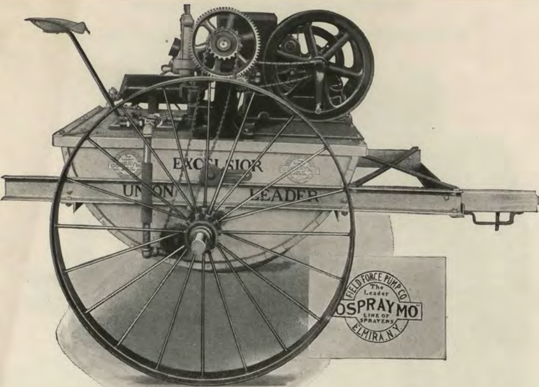
This shows a side view of the EXCELSIOR LEADER with the counter-shaft pump for High Speed Engines
