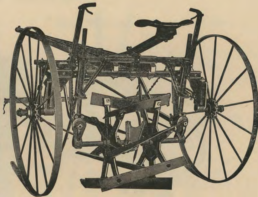
No. 50 Disc Cultivator, Equipped with Stalk Cutter Attachment
