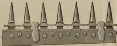
SECTION OF FINGER-BAR SHOWING CHAFE PLATES BETWEEN FINGERS.
