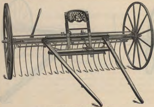
Standard 8-ft. Wood Rake with Thills.
