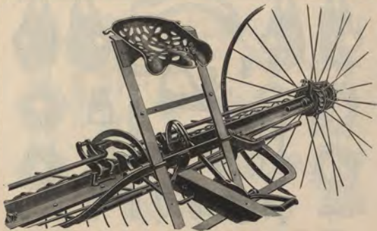
Enlarged View of Frame and Dumping Apparatus with New 20th Century Improvement.
