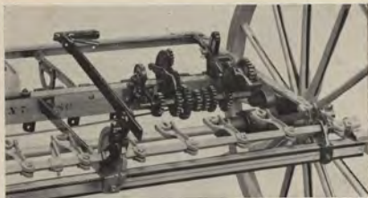
Countershaft with quantity gears and detail of frame, showing grain speed device—grass seeder gear stand—land measure—folding lever.
