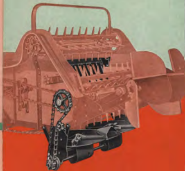
TWO-ROW CORN PICKER
