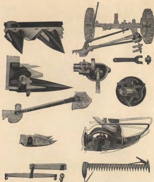
Serrated Guard Plate. Push Bar Raising Gag and Wide Main Frame. Showing Guard, Wear Plate and Oval Head Rivets. Pitman Connection. Ratchet Nut. Pitman. Pawl. Outer Shoe Sole Plate. Range of Tilt of Inner Shoe and Bar. Whiffletree Hooks and Chafing Plates. Underside of Cutting Bar.
