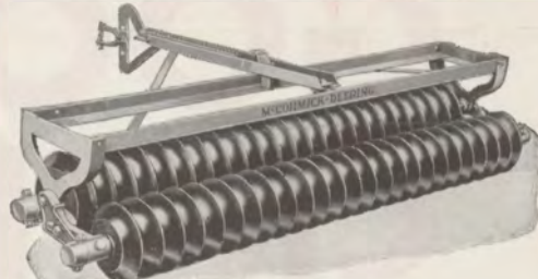
Illust. 22. McCormick-Deering double-gang soil pulverizer is supplied in a wide range of sizes for tractor or horse draft. It puts a real finish on a seed bed, crushing the clods and compacting the soil throughout the depth of the seed bed. The corrugations leave a nicely pulverized mulch on top. It is a handy tool to use behind a disk harrow.
