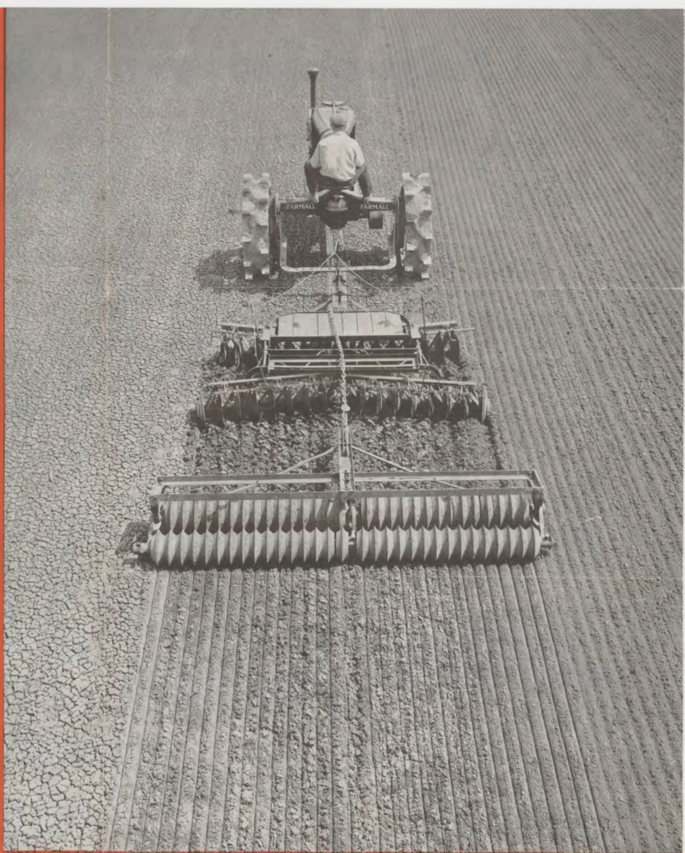
Illust. 1. The McCormick-Deering double-gang soil pulverizer does two important things—it makes the seed bed compact from top to bottom and it also breaks up crust and leaves the top soil loose enough to prevent subsurface moisture from escaping by evaporation. Because of the light draft it can be pulled easily in tandem behind another tool.
