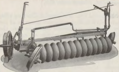
Illust. 11. The McCormick-Deering harrow-plow is supplied in 4, 5, 6, 8, and 9-foot sizes and is equipped with 20-inch deep-cut disks. The harrow-plow is a great weed killer and mulcher and therefore is a splendid implement for summer-fallow. Used immediately after harvest, it leaves the wheat stubble projecting from the soil, which greatly adds to the wind resistance of the soil.
