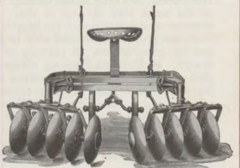
Illust. 18. McCormick-Deering reversible disk harrow. The disks can be set for in- or out-throw, which adapts this harrow to crop cultivation. It is available in 3, 4 and 5-foot sizes.
