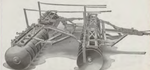
Illust. 13. The McCormick-Deering No. 9-A tractor disk harrow that has set new standards of long life, quick angling and accurate trailing—furnished in 5 to 10-foot sizes. The 9-B disk harrow has wide, 9-inch spacing between the disks. Similar disk harrows also are available with the weight boxes set below the level of the disks to facilitate close work under the trees in orchards.
