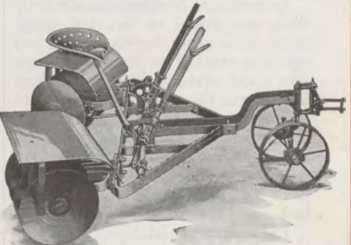
Illust. 17. McCormick-Deering orchard disk harrow. It is built in 4 and 5-foot sizes. An extension frame can be supplied on special order—it adds 49 inches to the over-all length.
