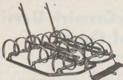
Illust. 8. McCormick-Deering 2-section, 17-tooth spring-tooth harrow with pipe bars. Channel steel bars also are available, as well as a variety of teeth to meet special conditions. Sizes from 2½ to 15 feet. Special quack grass harrows also are available.
