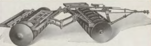
Illust. 14. McCormick-Deering No. 8-B offset tractor disk harrow. This harrow makes possible extremely close work in orchards and vineyards. It may be drawn directly behind the tractor or placed offset to either side and does a good job of disk even while turning. It may be turned easily either to the right or left. 5½ to 10½-foot sizes.
