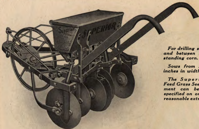
Superior Five Disc, One Horse, Plain Drill with Bale Hitch.
