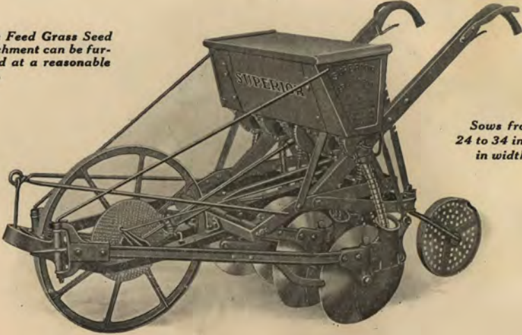
Superior Five Disc, One-Horse, Plain Grain Drill with Gauge Wheels.
