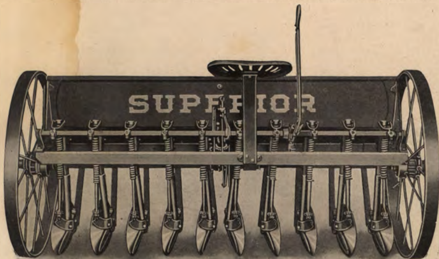
Superior 10x7 Single Disc Plain Drill with Seat and 4-foot Steel Wheels.
