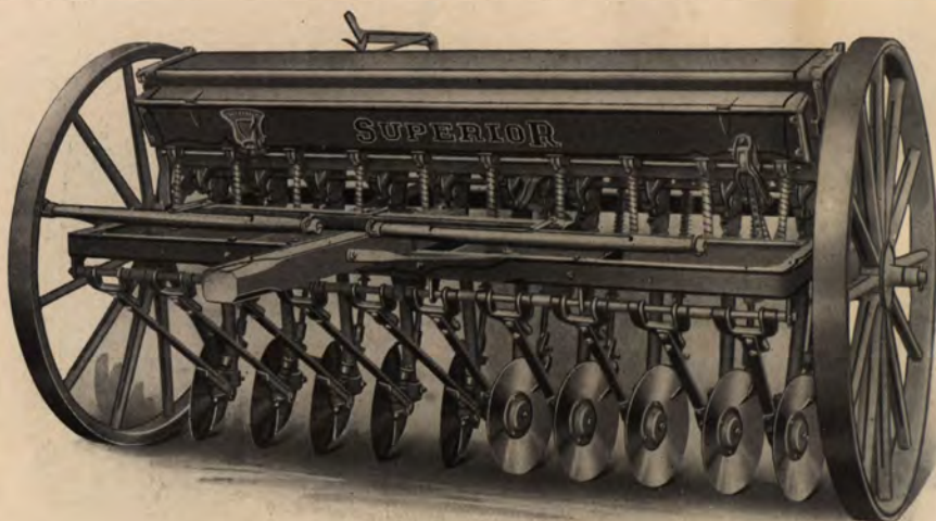
Front View Superior 10x8 Single Disc Fertilizer Drill with 4-foot Wood Wheels.
