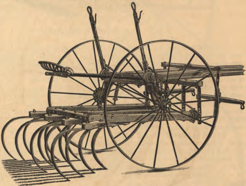
A Force Feed Seeding Attachment
