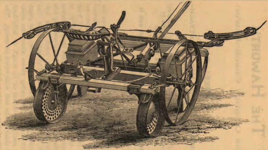
THE HAWORTH PLANTER WITH STEEL BAR.
