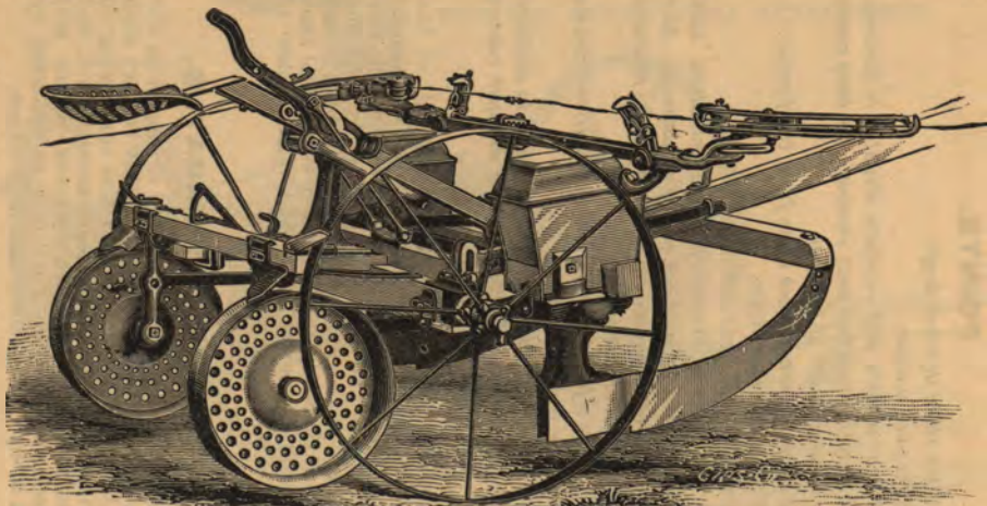
THE ABOVE CUT REPRESENTS THE PLANTER WITH THE REAR COVERING WHEELS AND RUNNERS ELEVATED FROM THE GROUND.
